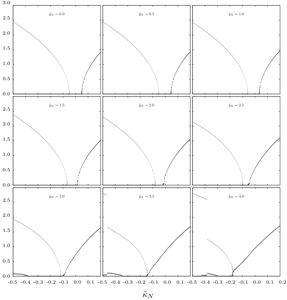
Figure 2: Expectation values for the amplitudes of the constant ( m : black curve) and staggered ( s : gray curve) modes for several selected values of the Yukawa coupling constant \tilde{y}_N and a constant quartic coupling \tilde{\lambda}_N = 0.3 . The results were obtained for L = \infty .
