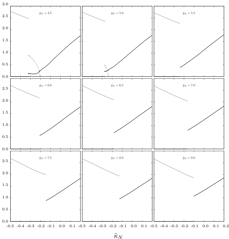
Figure 3: Expectation values for the amplitudes of the constant ( m : black curve) and staggered ( s : gray curve) modes for several selected values of the Yukawa coupling constant \tilde{y}_N and a constant quartic coupling \tilde{\lambda}_N = 0.3 . The results were obtained for L = \infty .
