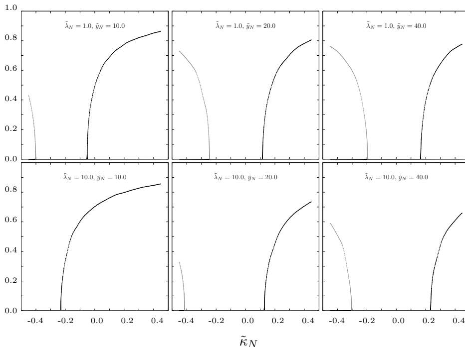
Figure 6: Expectation values for the amplitudes of the constant ( m : black curve) and staggered ( s : gray curve) modes for several selected values of the Yukawa coupling constant \tilde{y}_N and the quartic coupling parameters \tilde{\lambda}_N = 1.0 and \tilde{\lambda}_N = 10.0 . The results were obtained for L = \infty .
