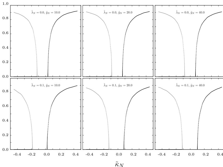
Figure 5: Expectation values for the amplitudes of the constant ( m : black curve) and staggered ( s : gray curve) modes for several selected values of the Yukawa coupling constant \tilde{y}_N and the quartic coupling parameters \tilde{\lambda}_N = 0.0 and \tilde{\lambda}_N = 0.1 . The results were obtained for L = \infty .
