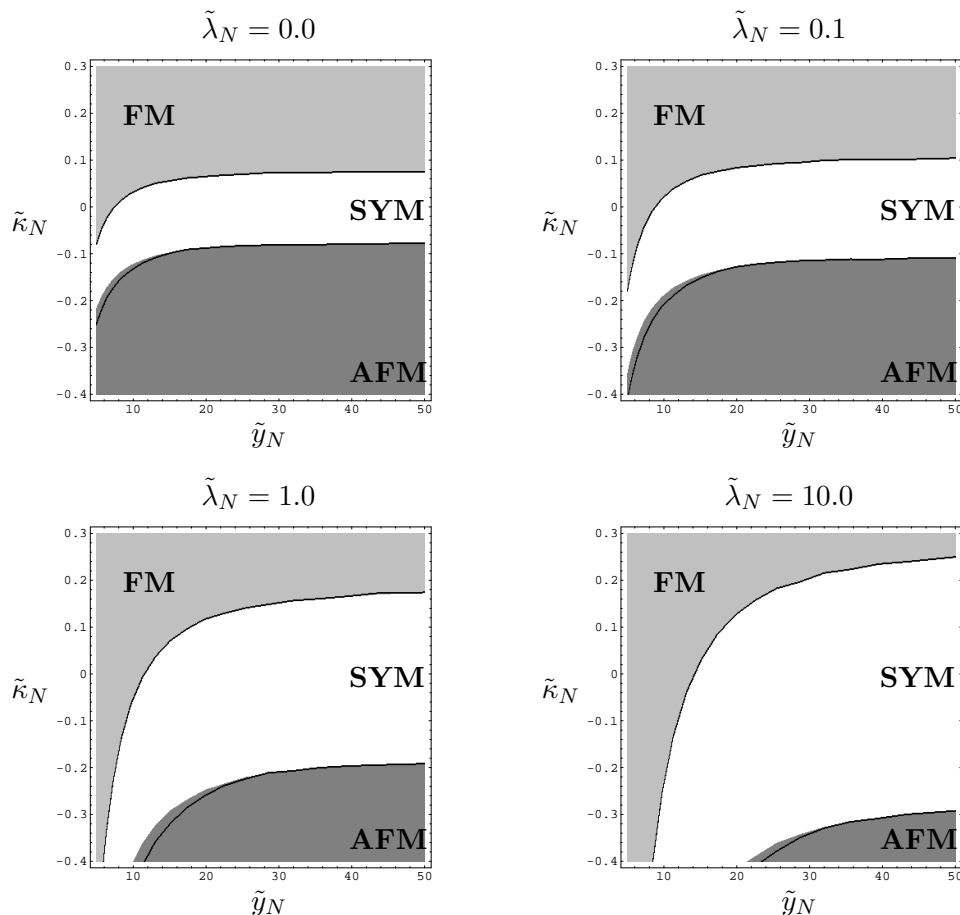
Figure 4: Phase diagrams for L = \infty with respect to the Yukawa coupling constant \tilde{y}_N and the hopping parameter \tilde{\kappa}_N for several selected values of the quartic coupling constant \tilde{\lambda}_N . The presented phase structure was determined for \epsilon = 10^{-1} , while the black lines show the phase transition lines obtained for \epsilon = 10^{-3} . An explanation of the \epsilon -dependence of the presented results is given in the text.
