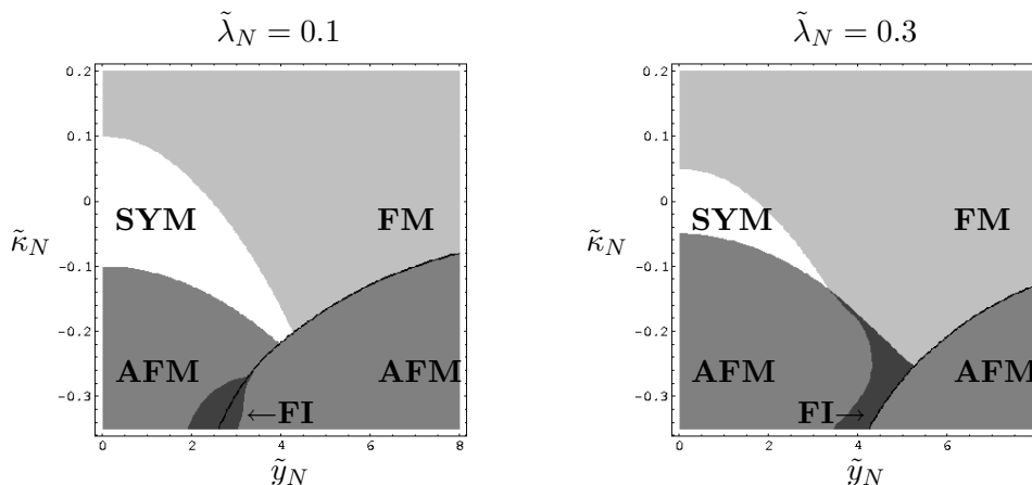
Figure 1: Phase diagrams with respect to the Yukawa coupling constant \tilde{y}_N and the hopping parameter \tilde{\kappa}_N for the constant quartic couplings \tilde{\lambda}_N = 0.1 (left) and \tilde{\lambda}_N = 0.3 (right). The black line indicates the first order phase transitions. Both phase diagrams were determined for L = \infty . An explanation of the occurring phases is given in the text.
